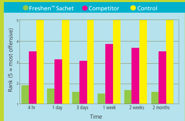
Fig. 2. Comparative panel test results show that Novozymes Freshen™ Sachet exhibits superior odor perception on urine malodors in four hours and continuously for two months compared to a competitor product.
