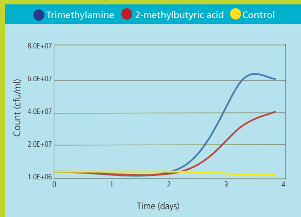
Fig. 3. Novozymes Freshen™ Sachet beneficial microorganism growth on two odorous molecules as the sole carbon source (2-methylbutyric acid and trimethylamine) after three days.
