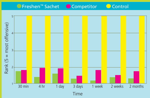
Fig. 1. Test demonstrates the capability of Novozymes Freshen™ Sachet to more effectively reduce urine malodors after only 30 minutes and continuously for as long as two months compared to a competitor product.
